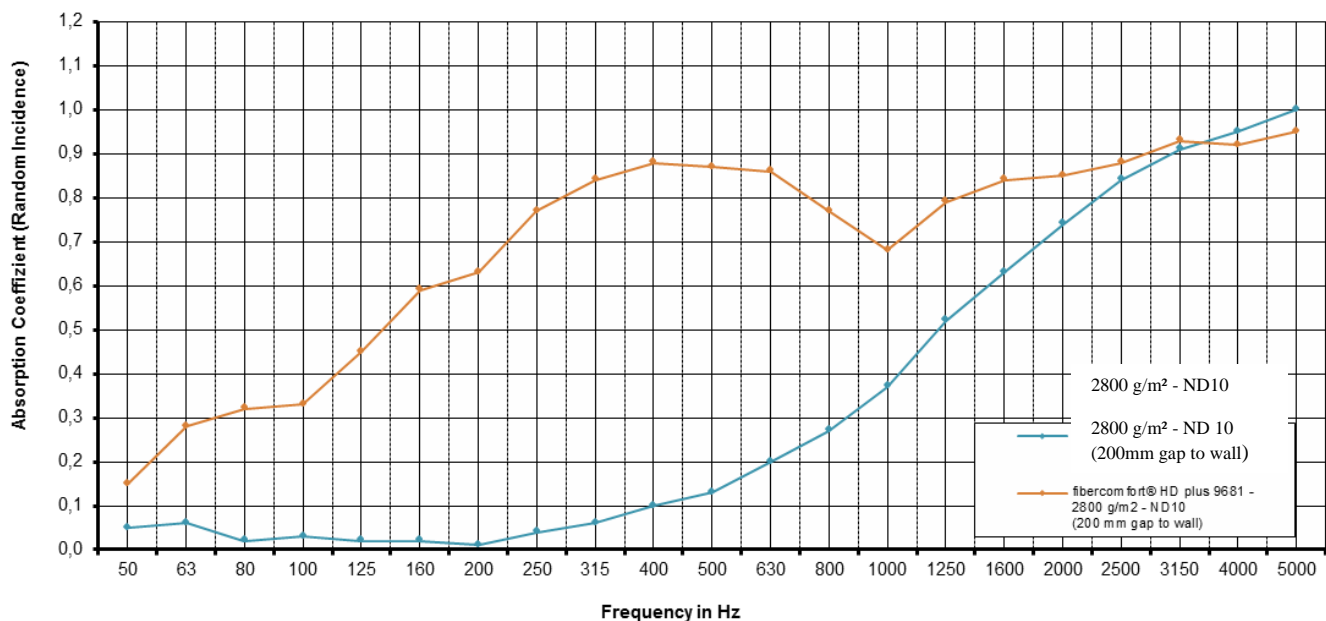
Measurement in a reverberation room - ISO 354:2003
