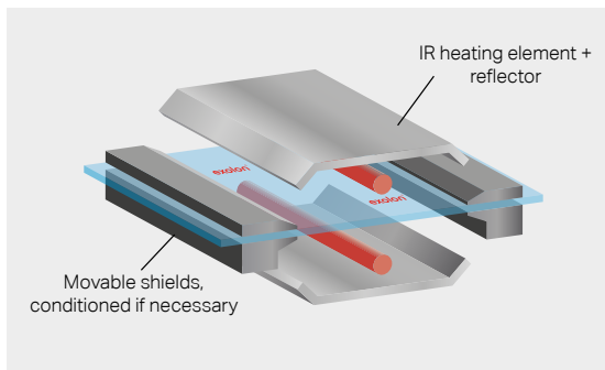
Hot folding
