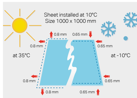
Thermal expansion
