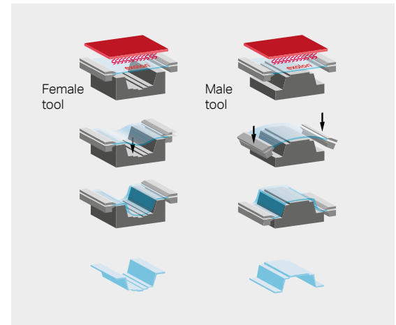
Sketch of vents during thermoforming
