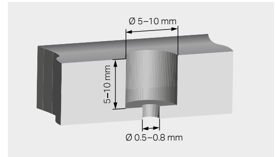
Sketch of vents during thermoforming
