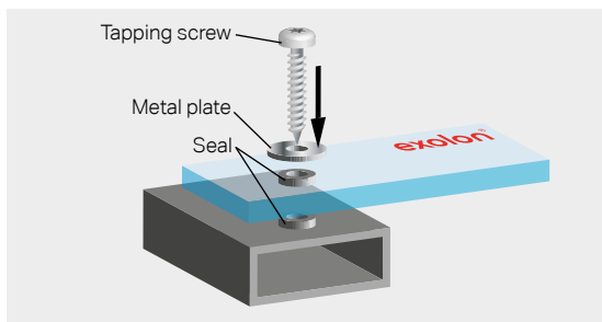
Mechanical fastening
