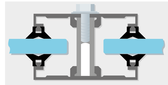
Distance ring
